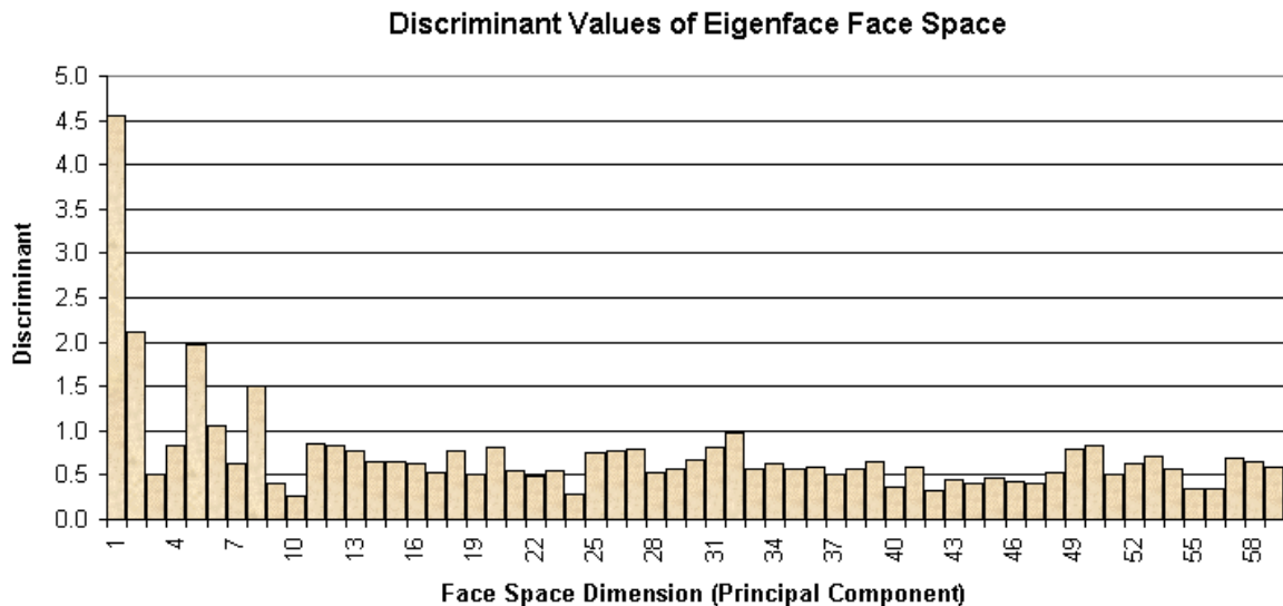
Fig. 4. Discriminant values of the eigenface face space dimensions using no image pre-processing.
