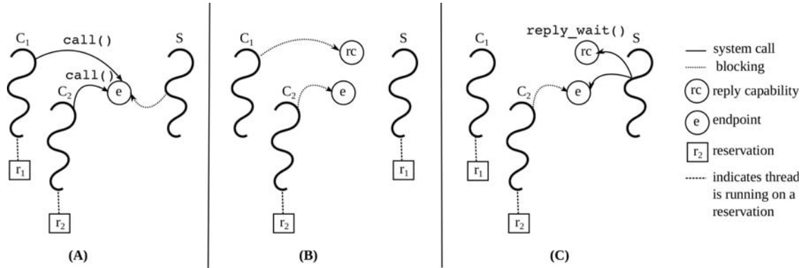
Fig. 1. Client threads invoke a passive server via IPC on endpoint e . In (A), two clients, ( C_1 and C_2 with reservations r_1 , r_2 ) both send requests to the server S via call() . In (B), C_1 's message is processed first: the kernel generates a one-shot endpoint ( rc ) that C_1 blocks on, and the server borrows C_1 's reservation r_1 while running on C_1 's behalf, while C_2 remains blocked on the endpoint. (C) shows S completing the invocation using reply_wait() on e , transferring r_1 back to C_1 over rc . Note that the system is strictly speaking never in the state shown in (C), as the reply_wait() operation is atomic, so S switches directly from the reply to C_1 (through rc ) to receiving the message and reservation from C_2 .
