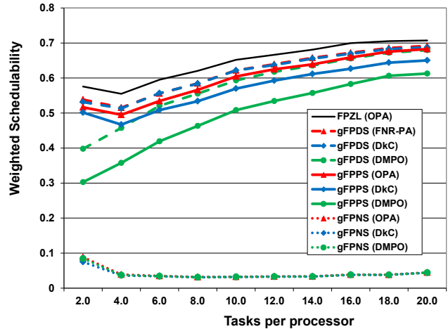
Figure 7: Weighted schedulability as a function of taskset size
