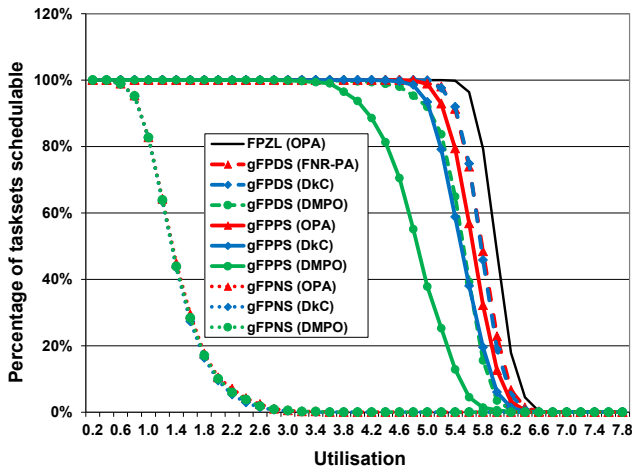
Figure 6: Success ratio for m = 8, n = 40, implicit deadlines
