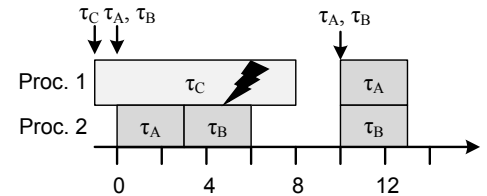
Figure 5: Schedule with gFPNS.
