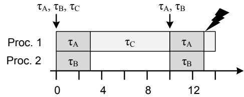
Figure 4: Schedule with gFPPS.
