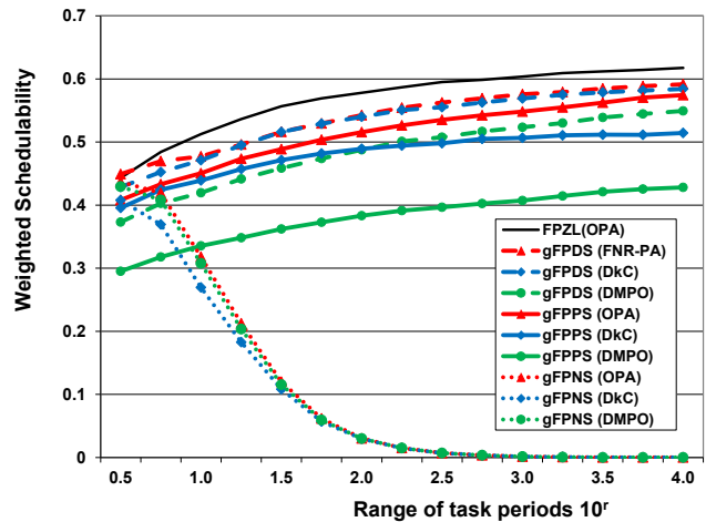
Figure 8: Weighted schedulability as a function of period range, D \leq T
