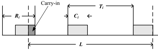
Figure 3: RTA analysis: Interference within an interval.
