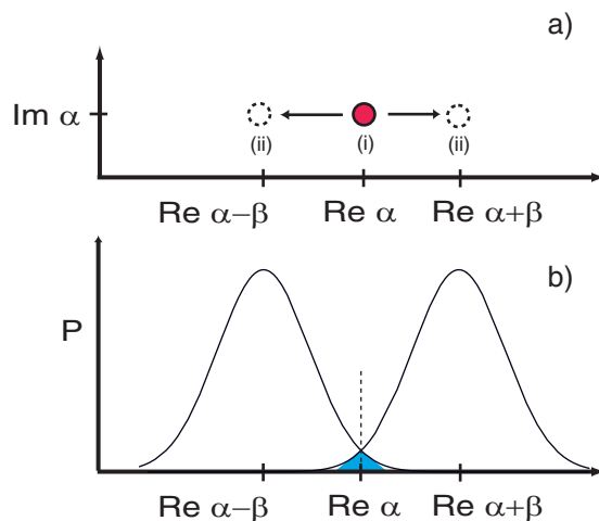
Figure 2. Schematic diagram showing the effect on the CV bus coherent state of interaction with the qubit (a). The coherent state is displaced conditional on the qubit state. The labels (i) and (ii) correspond to the evolution stages, as shown in the circuit diagram in the previous figure. (b) A schematic diagram of the X(0) quadrature probability distribution for the CV bus mode state after interaction with the qubit. Clearly, the qubit measurement is not perfect due to the overlap of peaks corresponding to different computational basis states.
