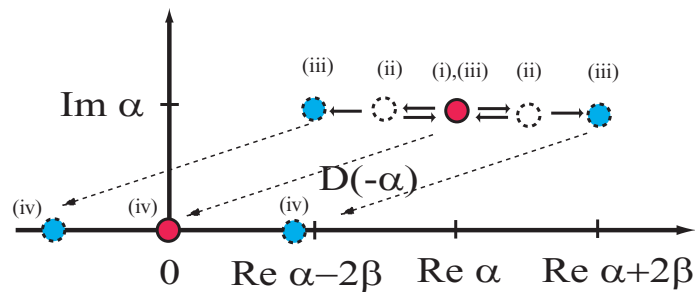
Figure 4. Schematic diagram showing the phase space evolution of the bus amplitudes corresponding to the various qubit computational basis states. The labels (i)–(iv) correspond to the evolution stages, as shown in the circuit diagram in figure 3.
