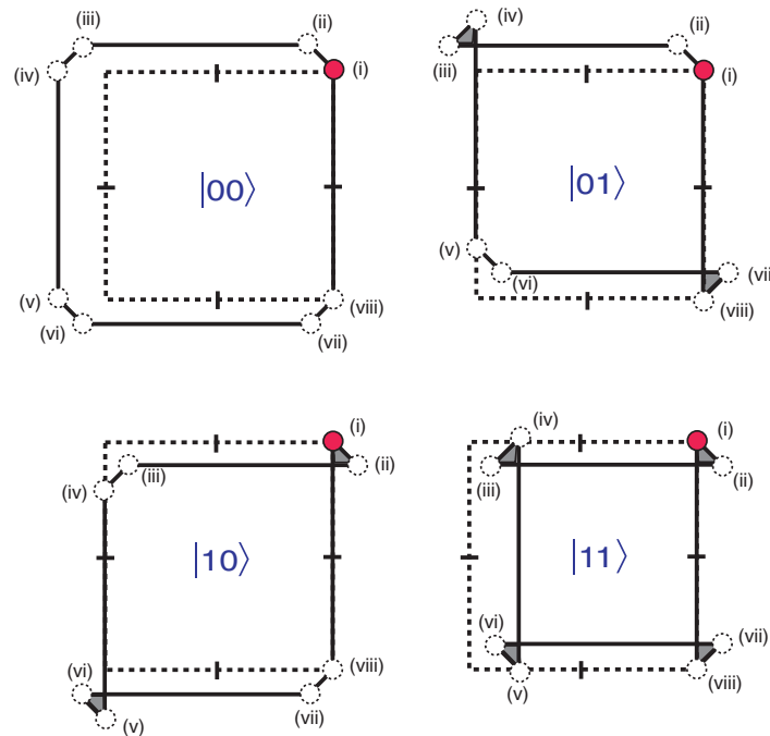
Figure 15. Schematic diagram showing the phase space evolution of the bus amplitudes corresponding to the various qubit computational basis states. The labels (i)–(viii) correspond to the evolution stages, as shown in the circuit diagram in the previous figure. The small areas shown in grey are traversed in a clockwise sense, giving a negative contribution to the phase acquired.
