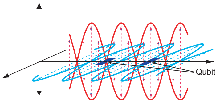
Figure 9. Schematic diagram of an array of planar charge qubits coupled to a common microwave bus mode. Adjacent qubits are respectively coupled to the antinode of the electric field (across the junction) and the antinode of the magnetic field (threading the composite junction loop), enabling the forms of coupling needed for the measurement-free gate.
