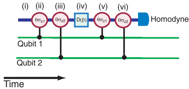
Figure 12. The circuit diagram for a two-qubit parity gate based on controlled rotations between the qubits and the probe bus, followed by bus X(0) quadrature measurement. The amplitude of the unconditional displacement is given by \beta = -2\alpha \cos 2\theta .
