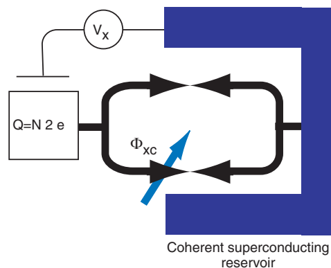
Figure 7. Schematic diagram of a charge qubit. A superconducting island with excess charge 2Ne is connected to a reservoir through a composite Josephson junction, whose effective tunnelling amplitude is controlled by the magnetic flux \Phi_{xc} . An external voltage bias V_x is applied to induce an additional polarization charge.
