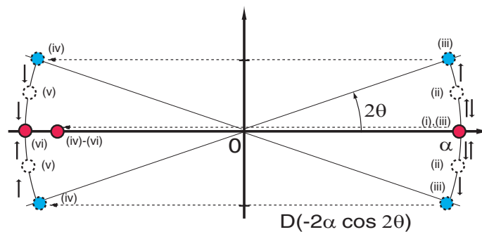
Figure 13. Schematic diagram showing the phase space evolution of the bus amplitudes corresponding to the various qubit computational basis states. The labels (i)–(vi) correspond to the evolution stages, as shown in the circuit diagram in the previous figure.
