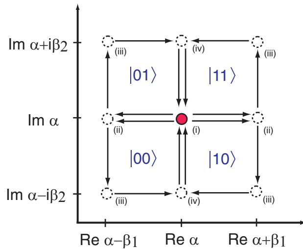
Figure 6. Schematic diagram showing the phase space evolution of the bus amplitudes for the four basis states of the two qubits. The labels (i)–(iv) correspond to the evolution stages, as shown in the circuit diagram in figure 5.
