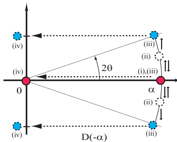
Figure 11. Schematic diagram showing the phase space evolution of the bus amplitudes corresponding to the various qubit computational basis states. The labels (i)–(iv) correspond to the evolution stages, as shown in the circuit diagram in the previous figure.
