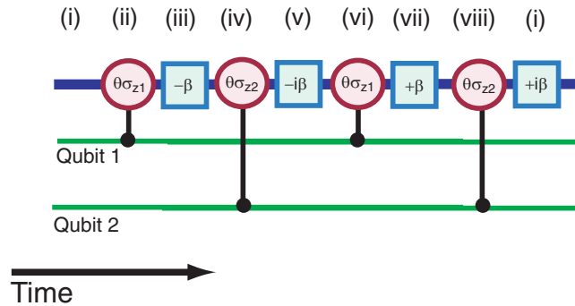
Figure 14. The circuit diagram of a two-qubit controlled-phase gate, based on controlled rotations between the qubits and the probe bus and non-controlled displacements of the bus.
