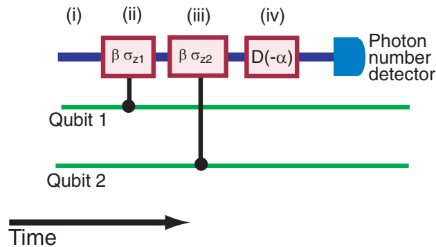
Figure 3. Circuit diagram for a two-qubit parity gate based on controlled displacements between the qubits and the ‘probe’ bus, followed by bus measurement.
