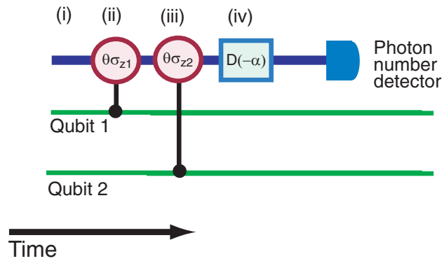
Figure 10. The circuit diagram for a two-qubit parity gate based on controlled rotations between the qubits and the probe bus, followed by bus number measurement.
