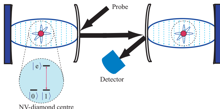
Figure 16. Schematic diagram of a two NV-diamond centre qubits in separate cavities coupled via a cross-kerr interaction to an optical field. The final measurement enables the construction of a parity gate.
