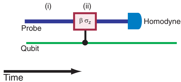
Figure 1. Circuit diagram for the QND measurement scheme based on conditional displacement of the bus mode by the qubit followed by a homodyne measurement on the bus mode.
