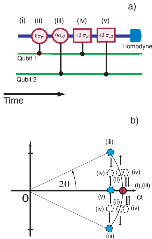
Figure 17. (a) The circuit diagram of a two-qubit parity gate, based on controlled rotations and controlled displacements between the qubits and the probe bus. (b) Schematic diagram showing the phase space evolution of the bus amplitudes corresponding to the various qubit computational basis states. The labels (i)–(v) correspond to the evolution stages, as shown in the circuit diagram in (a).
