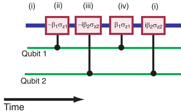
Figure 5. Circuit diagram of a universal two-qubit gate based on controlled displacements between the qubits and the ‘probe’ bus.
