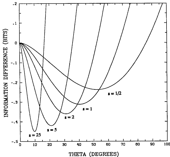
FIG. 1. Information difference \mathcal{H}^{\text{QM}}(\theta) in bits vs angle \theta in degrees for s = \frac{1}{2} , 1, 2, 5, and 25. The maximum information deficit for s = \frac{1}{2} is -0.2369 bits at 52.31^\circ ; for s = 25 , -0.4493 bits at 9.798^\circ .
