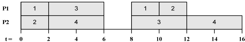
Figure 1: Critical instant effect
