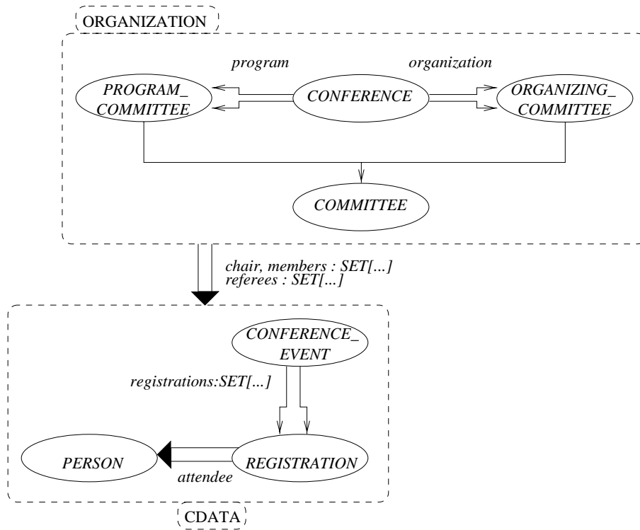
Fig. 16: Client relations involving clusters
