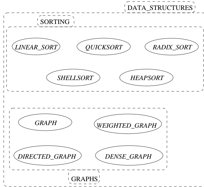
Fig. 13: A nested cluster
