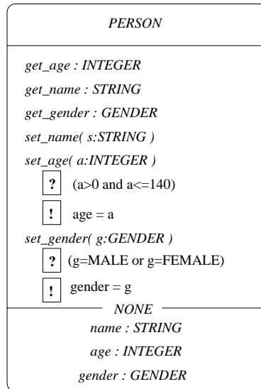
Fig. 6: Class PERSON annotated with contracts and types
