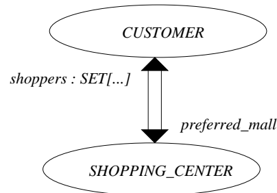
Fig. 15: Bidirectional association links
