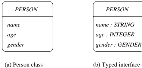
Fig. 1: Variants of a person class
