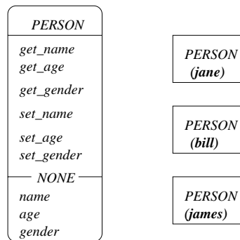
Fig. 5: Objects associated with class PERSON
