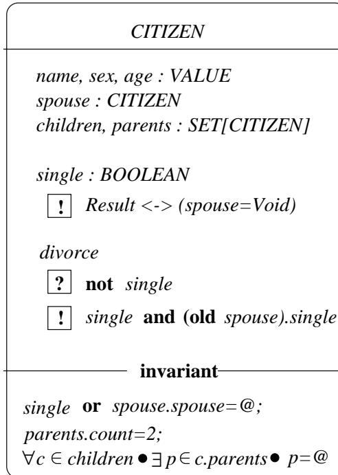
Fig. 7: BON graphical specification
