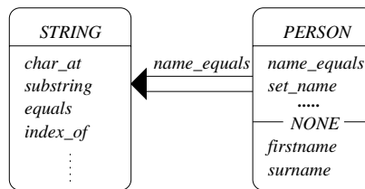
Fig. 11: Association, use of routine
