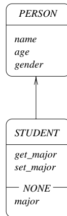
Fig. 9: Detailed view, with inheritance
