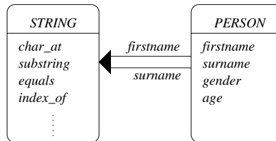
Fig. 10: Association relationship between two classes
