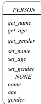
Fig. 4: Class with public routines, private attributes
