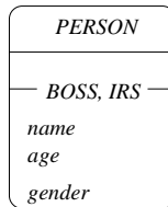
Fig. 3: Class with an access list
