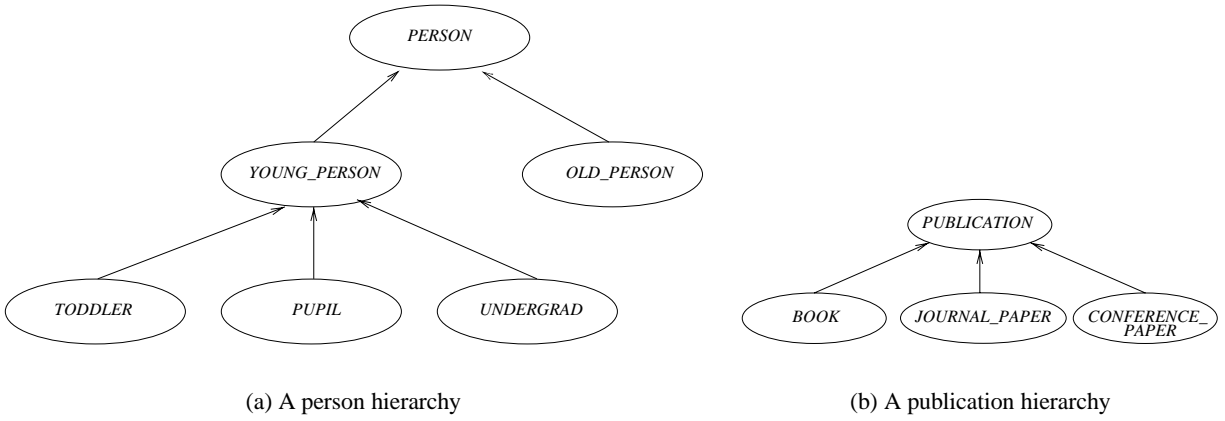
Fig. 8: Inheritance diagrams in BON
