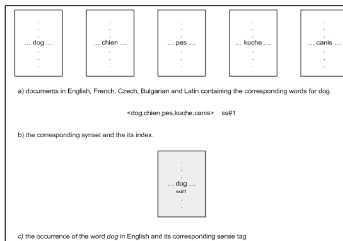
Fig. 2: Assignment of sense tags in aligned documents.
