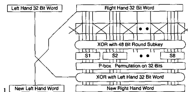
Fig. 1. Round of Data Encryption Standard
