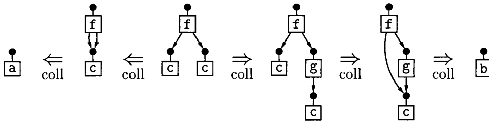
FIG. 9. Nonconfluence of \Rightarrow_{\text{coll}} and \Rightarrow_{\text{bi}} .
