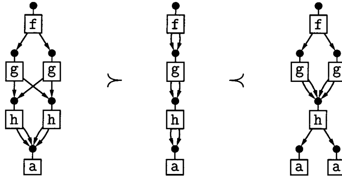
FIG. 1. Collapsing and copying.
