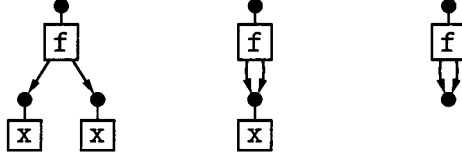
FIG. 2. The graphs \Delta^f(x, x) , \diamond f(x, x) and \underline{\underline{\diamond f(x, x)}} .
