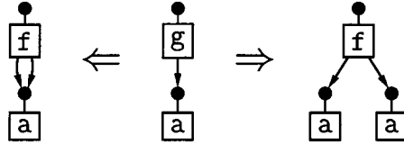
FIG. 8. Church–Rosser property modulo \sim without confluence.
