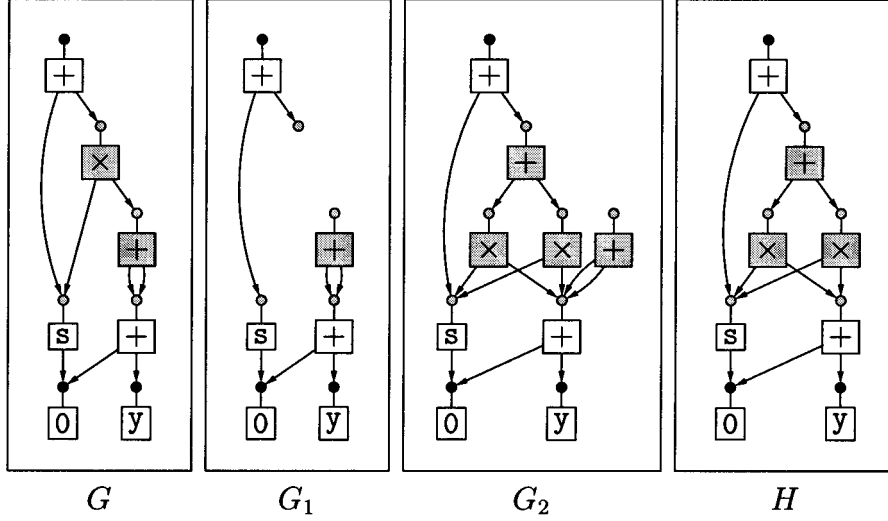
FIG. 3. The construction of a term graph rewrite step.
