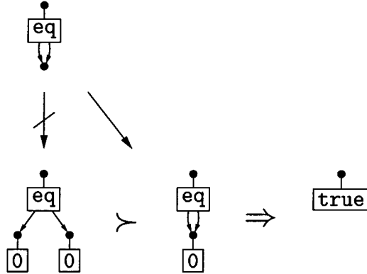
FIG. 4. Collapsing to enable a rule application.
