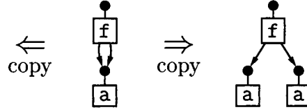
FIG. 10. Nonconfluence of \Rightarrow_{\text{copy}} .
