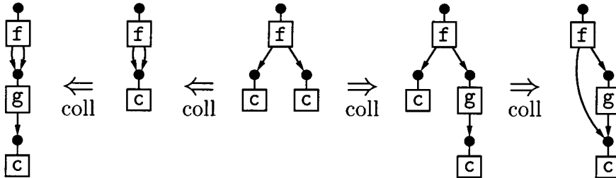
FIG. 11. Nonconfluence of \Rightarrow_{\text{coll}} .
