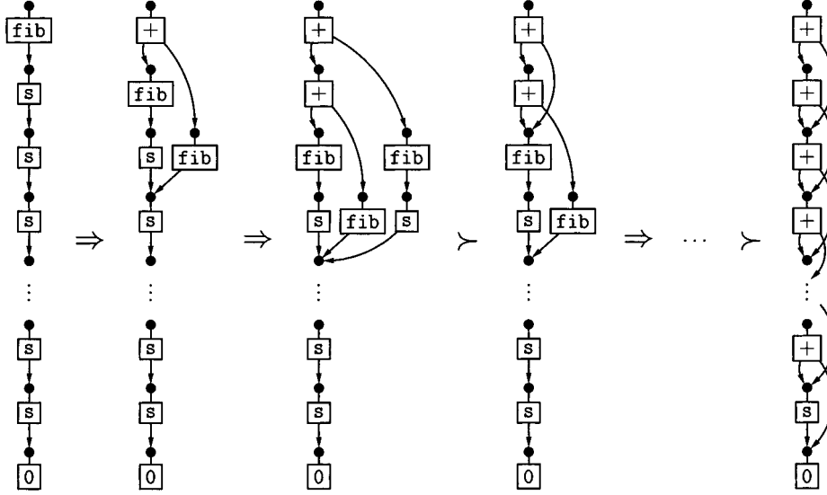
FIG. 5. Collapsing to speed up evaluation.
