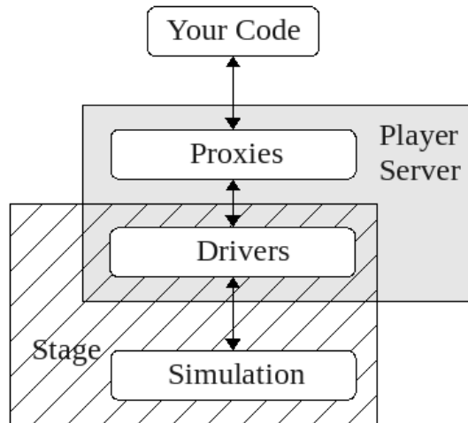
Figure 20: The server/client control structure of Player/Stage when used as a simulator. There may be several proxies connected to the server at any time.
