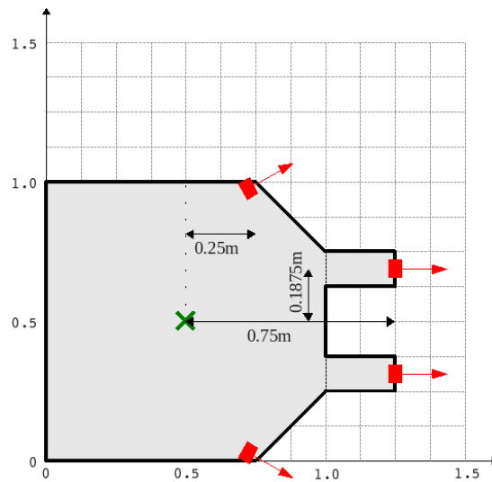
Figure 12: The position of Bigbob's sonars (in red) relative to its origin. The origin is marked with a cross, some of the distances from the origin to the sensors have been marked. The remaining distances can be done by inspection.
