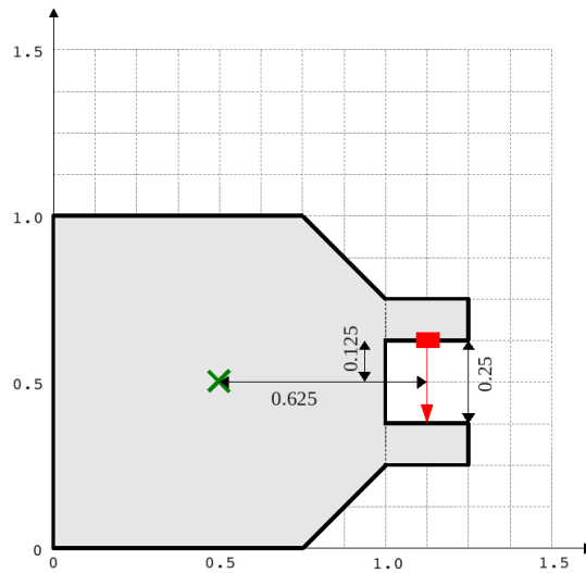
Figure 13: The position of Bigbob's laser (in red) and its distance, in metres, relative to its origin (marked with a cross).
