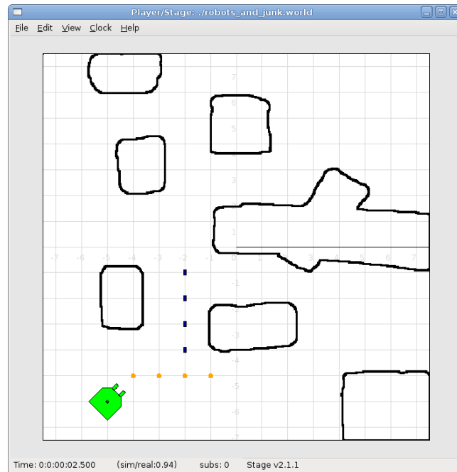
Figure 18: The Bigbob robot placed in the simulation along with junk for it to pick up.
