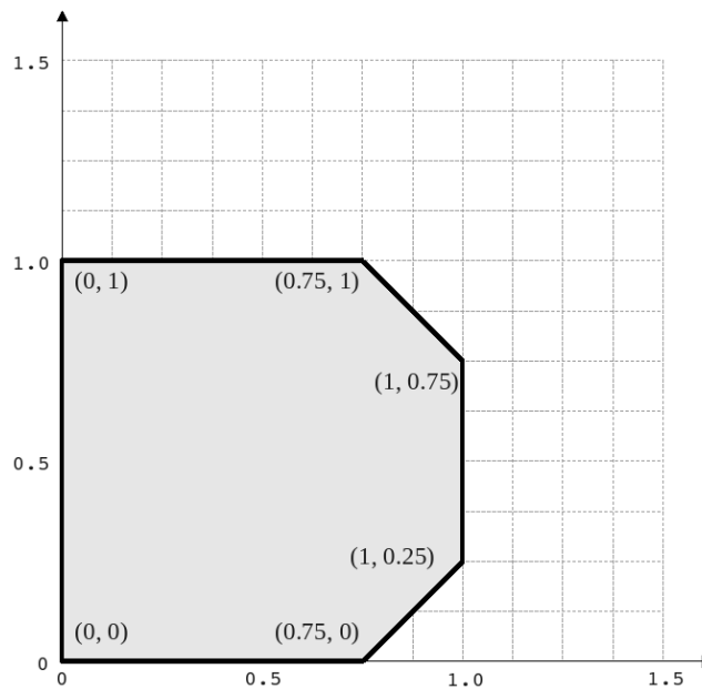
Figure 8: The basic shape we want to make Bigbob, the units on the axes are in metres.
