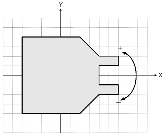
Figure 21: A robot on a cartesian grid. This shows what directions the X and Y speeds will cause the robot to move in. A positive yaw speed will turn the robot in the direction of the + arrow, a negative yaw speed is the direction of the - arrow.
